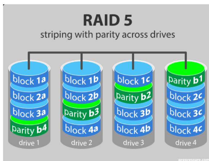
Figure 6 : RAID 5
